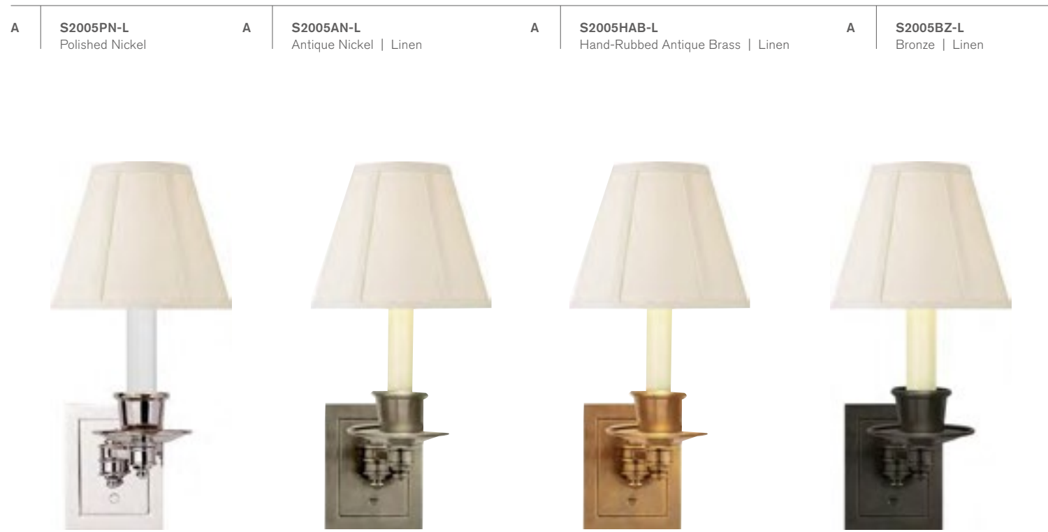
A SINGLE SWING ARM SCONCE STUDIO VC S2005 H: 12" | W: 6" | Ext: 7" Backplate: 3.5" x 4.5" Rec. Socket: E12 Candelabra | Bulb: 40 B Shade: 3" x 6" x 5" * Requires Smaller Outlet Box
