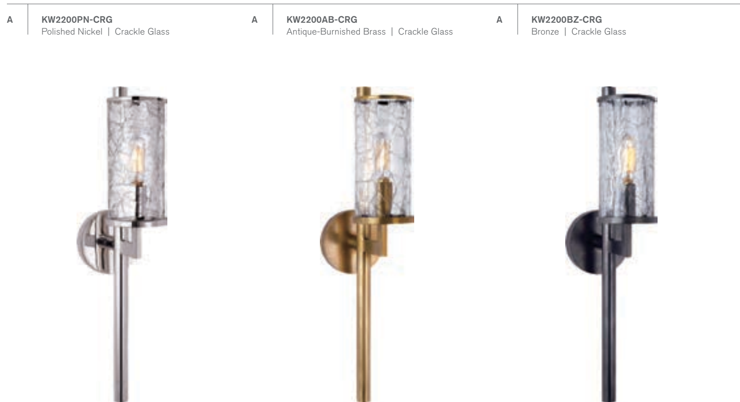
A LIAISON SINGLE ARM SCONCE KELLY WEARSTLER KW2200 H: 19" | W: 4" | Ext: 7.5" Backplate: 4" Round Socket: E12 Candelabra | Bulb: 60 C * Requires Smaller Outlet Box
