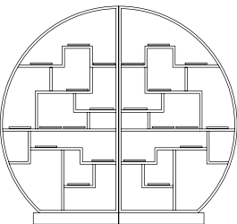
PSY.241.ALX L 250 D 45 H 230 cm
