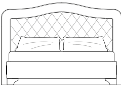
KIM.312.A bed for mattress L 180 D 200 cm L 219 D 213 H 142 cm
