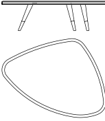
CAM.232.B central table L 145 D 115 H 35 cm
