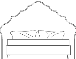
MAR.312.A bed for mattress L 180 D 200 cm L 222 D 212 H 172 cm
