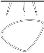
CAM.232.C central table L 145 D 115 H 40 cm
