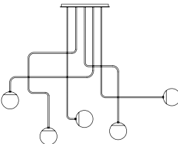
MAL.615.A 5-light chandelier L 140 D 18 H 110 cm
