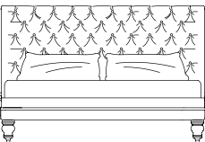
ALS.312.A bed for mattress L 180 D 200 cm L 190 D 239 H 125 cm
